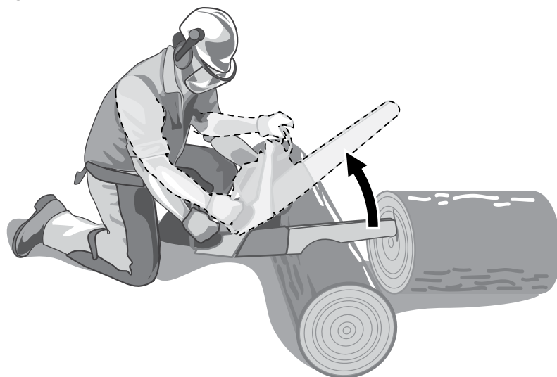
Figure 2. Chain saw kickback
